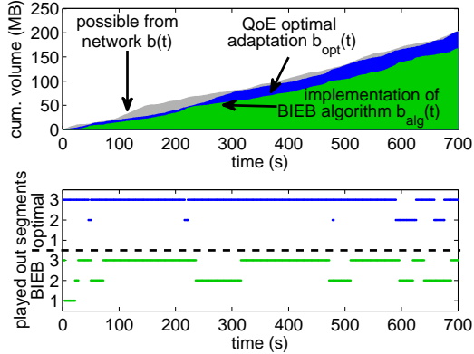
Figure 6: Single experiment comparing BIEB algorithm with theoretical QoE optimal adaptation strategy for the network scenario sketched in Figure 2.
