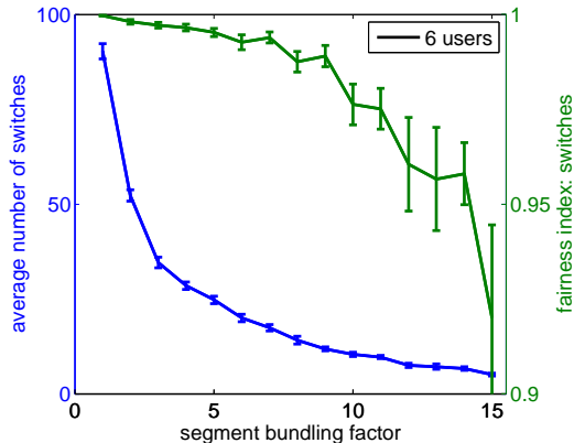
Figure 10: Influence of the segment bundling factor on the average number of switches and fairness in terms of switches for a multiple user scenario with U = 6 users.
