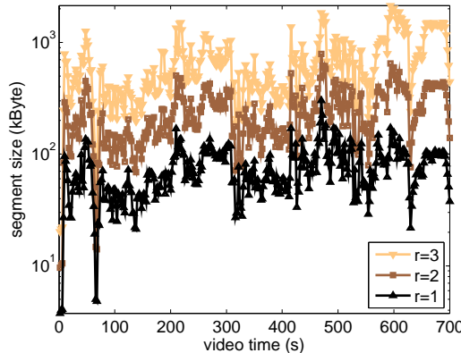
Figure 1: Segment sizes of the 3 representation layers for the example video of duration 700s used for the numerical results. The segment sizes are plotted on a logarithmic scale and sum up to 238.57 MB, 84.86 MB, 26.52 MB for r = 3, 2, 1 .
