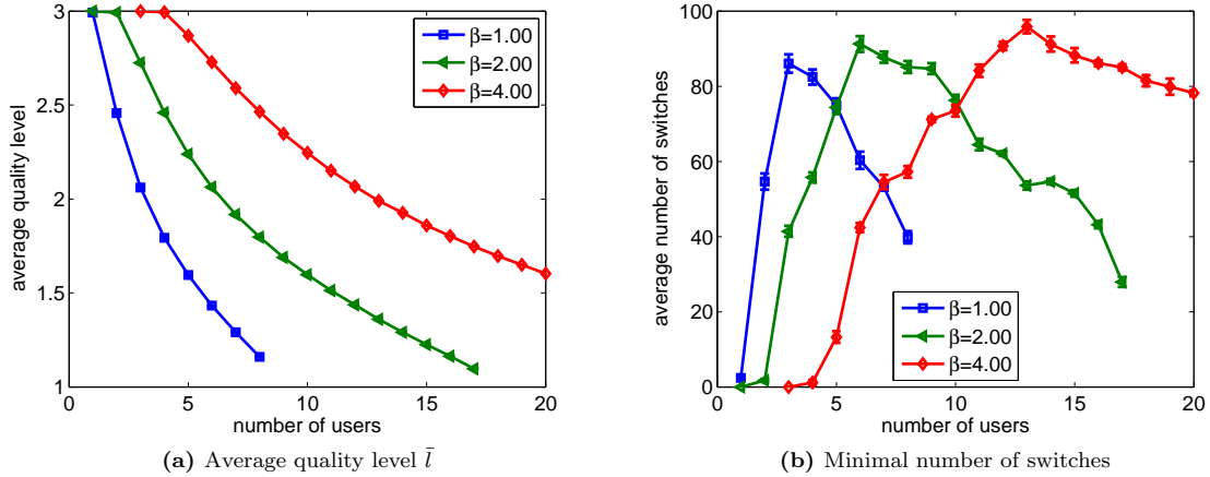
Figure 8: Optimal solution in multi-user IPTV scenario with service provisioning.
