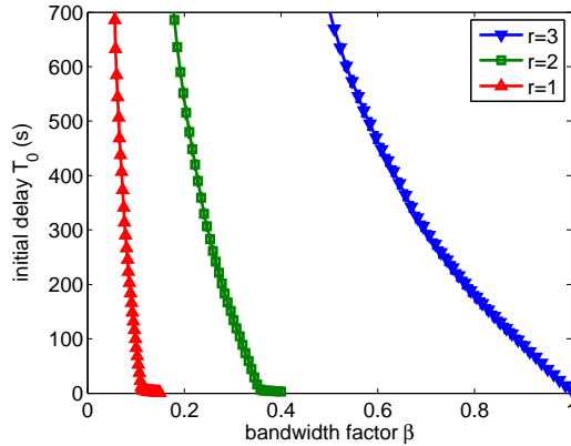
Figure 4: Optimal initial delay T_0 to download the video contents of representation r \in \{1, 2, 3\} without any stalling of the video playback.
