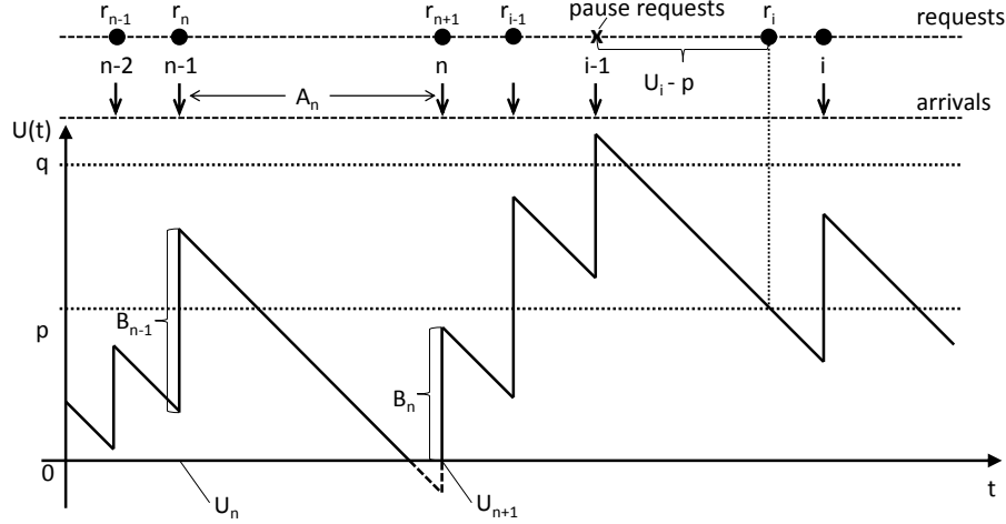
Fig. 2. Sample state process of GI/GI/1 buffer with pq -policy.
