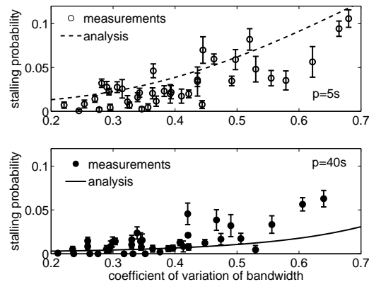
Fig. 8. Stalling probability of sample video in mobile throughput traces.
