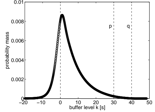
Fig. 3. Computational diagram for GI/GI/1 buffer with pq -policy. Fig. 4. Example probability mass of the buffer level distribution with negative buffer levels \hat{u}_n(k) .
