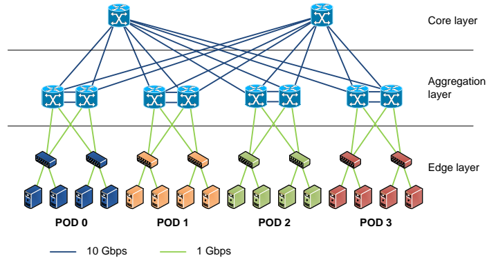
Fig. 2. Three-tier data center architecture.
