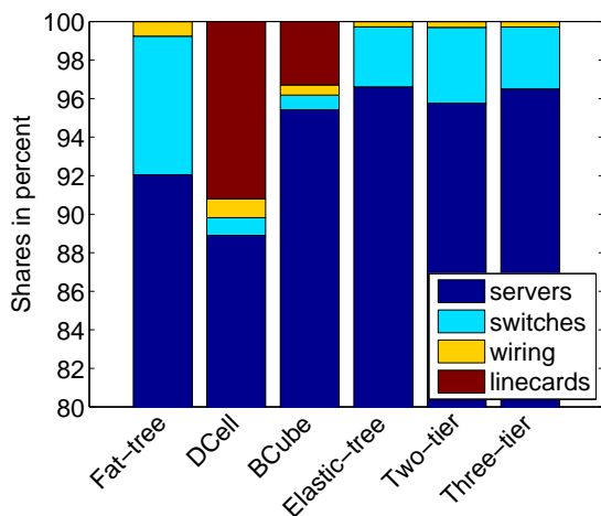
Fig. 8. Relative total power consumption.
