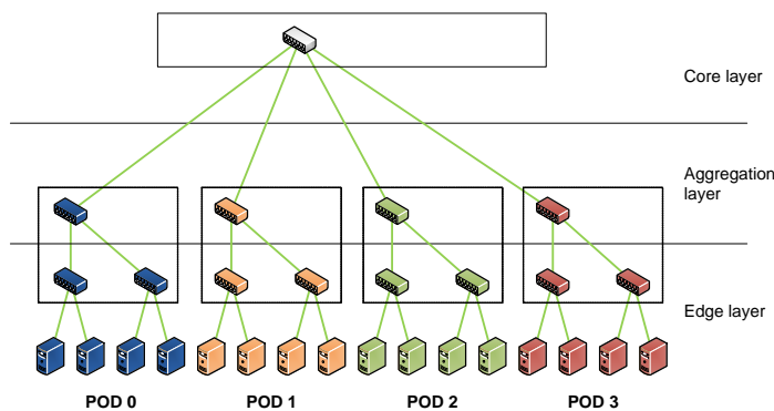
Fig. 6. Elastic-tree data center architecture.
