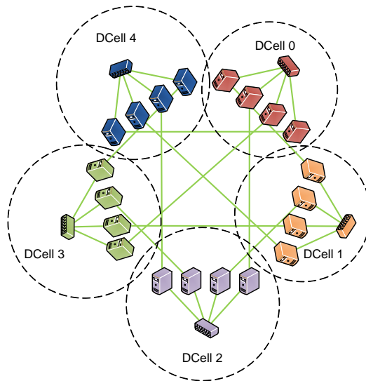
Fig. 3. DCell data center architecture.
