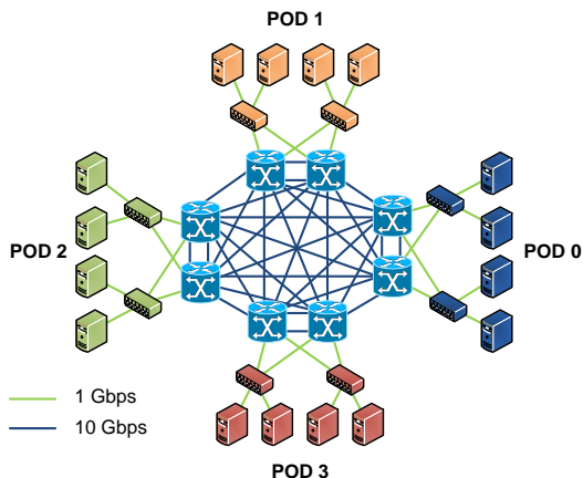
Fig. 1. Two-tier data center architecture.
