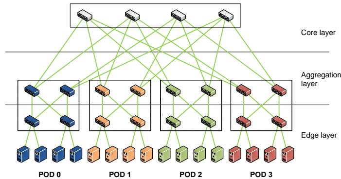
Fig. 5. Fat-tree data center architecture.
