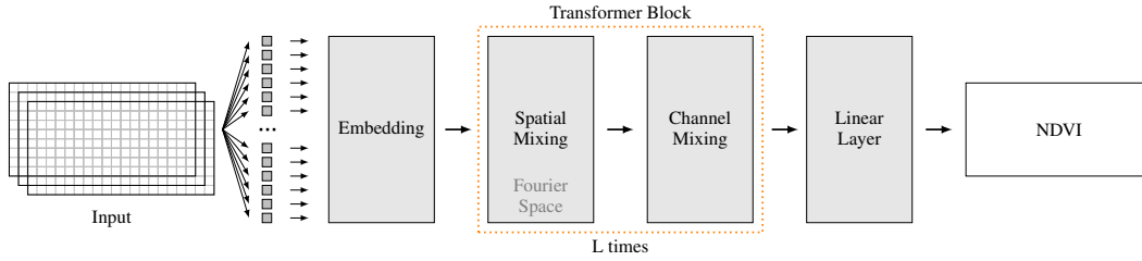
Figure 3: Overview of the used architecture based on the FourCastNet model Pathak et al. (2022). We initialize the model from pre-trained weights Pathak et al. (2023) and replace the weather-specific head with a linear head for modelling the normalized difference vegetation index (NDVI).
