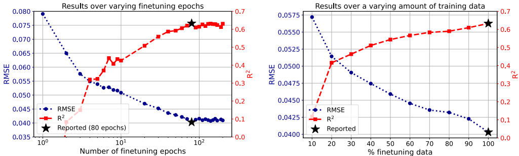
Figure 1: Results for ablation studies I & II. Left: varying number of finetuning epochs. Right: Varying amount of training data. Results reported in Table 1 are highlighted in both plots.
