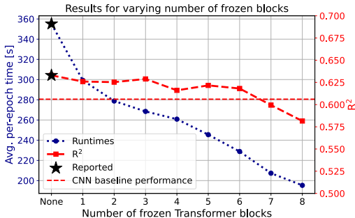
Figure 2: Results for ablation study III: varying number of frozen Transformer blocks during finetuning. Runtimes are averaged over five epochs.
