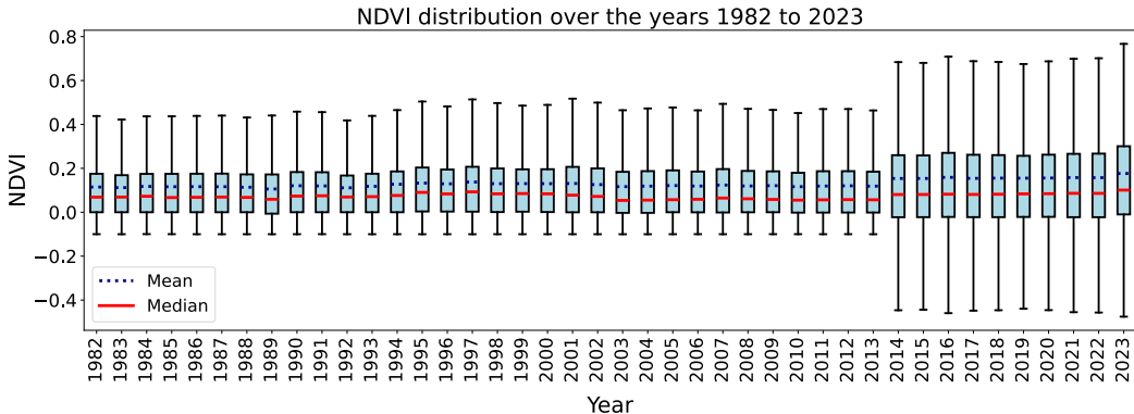
Figure 5: Distribution of the normalized difference vegetation index (NDVI) data from 1982 to 2023. NDVI data was only used until 2013 due to the noticeable data shift afterwards.
