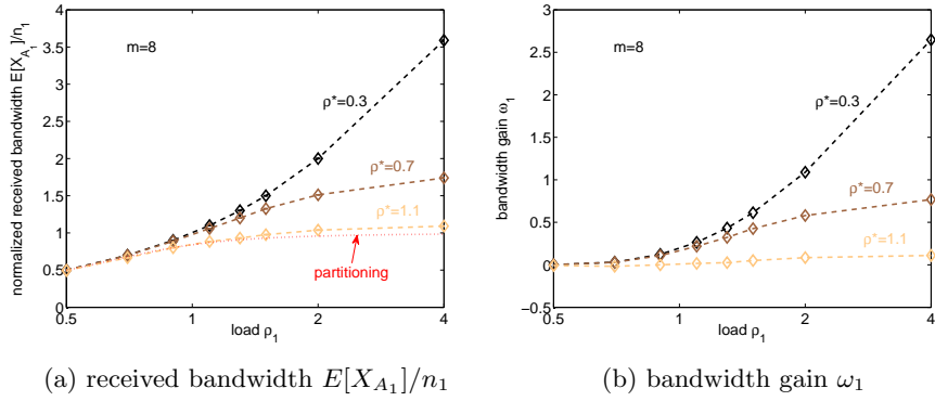
Figure 10: Received bandwidth and bandwidth gain dependent on throughput of cooperating systems \rho^* for m = 8
