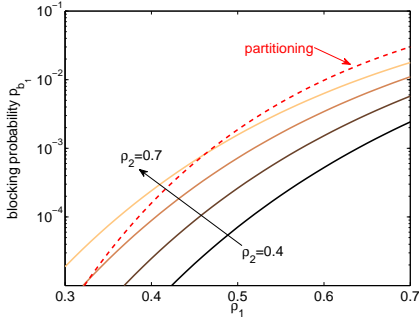
Figure 5: Blocking probability p_{b_1} dependent on load and load on cooperating system.
