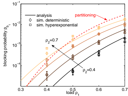
Figure 8: Blocking probability p_{b_1} dependent on load. Simulation with different service time distributions.
