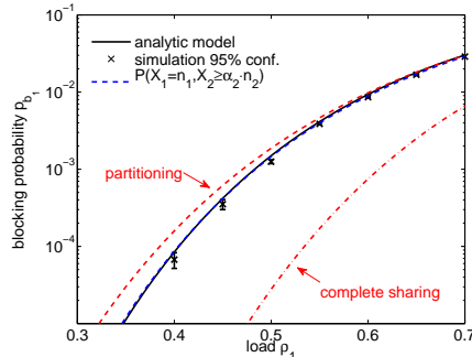
Figure 3: Blocking probability of two systems with equal load.
