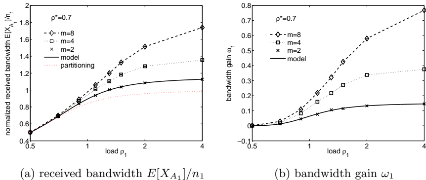
Figure 9: Received bandwidth and bandwidth gain dependent on number of cooperating systems m for \rho^* = 0.7
