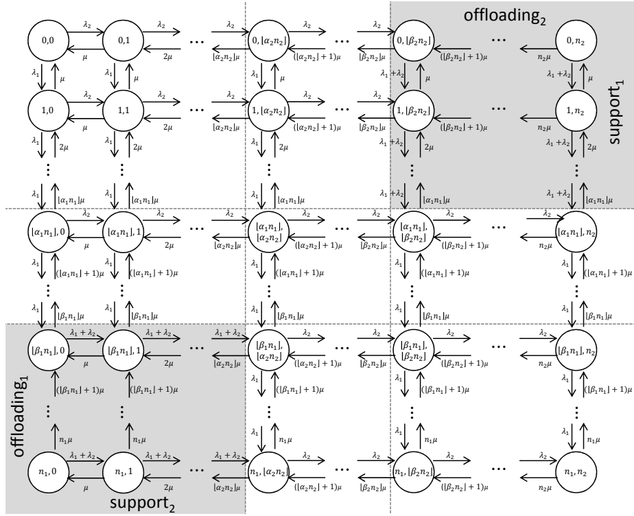
Figure 2: The state transition diagram.
