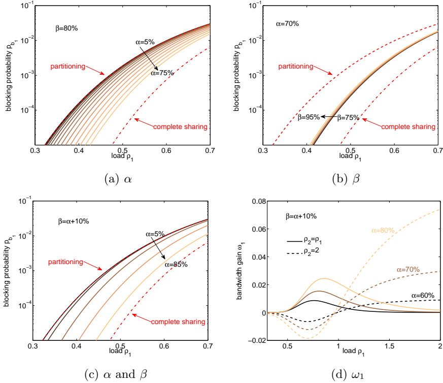
Figure 4: Blocking probability p_{b_1} dependent on thresholds (a) \alpha , (b) \beta and (c) \alpha and \beta , and (d) bandwidth gain \omega_1 .
