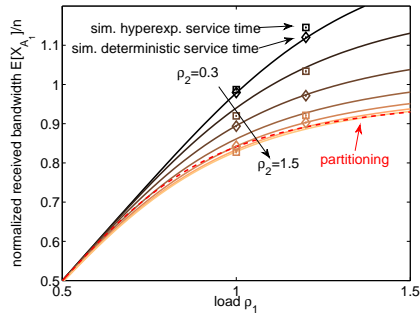
Figure 7: Normalized received bandwidth dependent on the load of reference and cooperating system.
