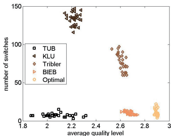
Fig. 7: Scatter plot for the 30 trial runs: average quality level vs. number of switches for the different adaptation algorithms and the optimal solution.
