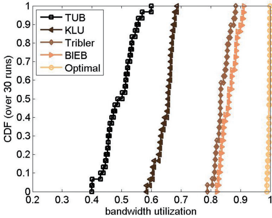
Fig. 3: Bandwidth utilization.
