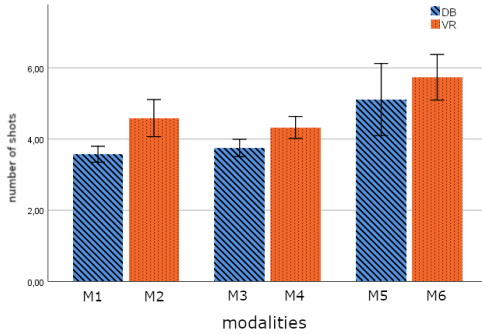
Fig. 7. Number of shots of all six modalities.
