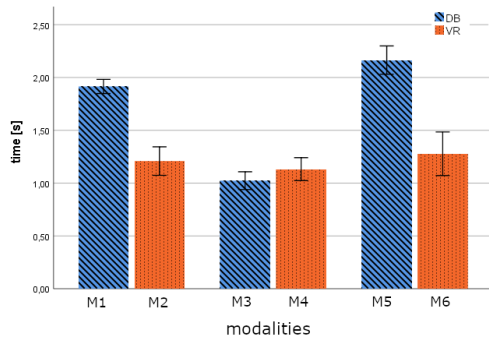
Fig. 4. Target acquisition times of all six modalities.
