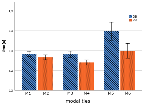
Fig. 5. Pointing times of all six modalities.
