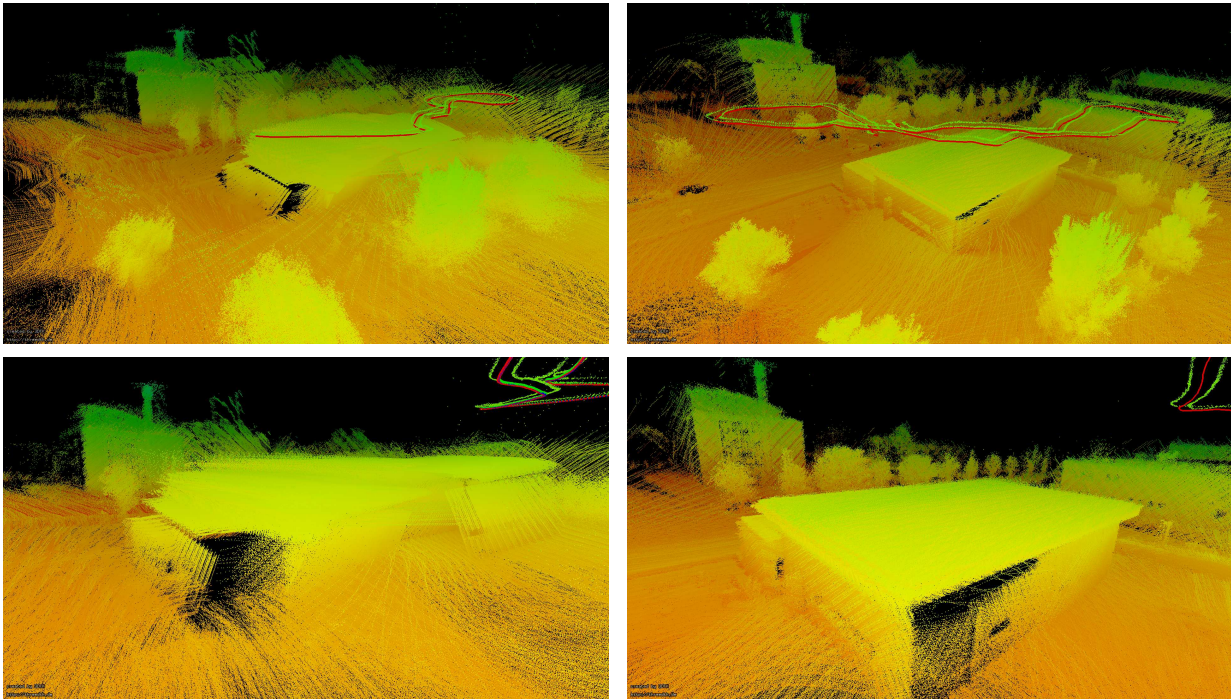
Fig. 2: Left: 3D point cloud with initial trajectory estimation. Note, that the highest position error is in the up axis. Right: Point cloud after applying semi rigid ICP with loop closing.
