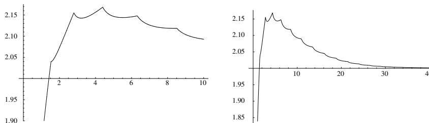
Fig. 7. The competitive ratio as a function of d : (Left) for small values of d . (Right) for larger values of d . Note the cusps at threshold values, the sharp peak at (4.4, 2.17) , and the clear asymptotic behavior. The first step length, x_1 , is given by c - 1 .
