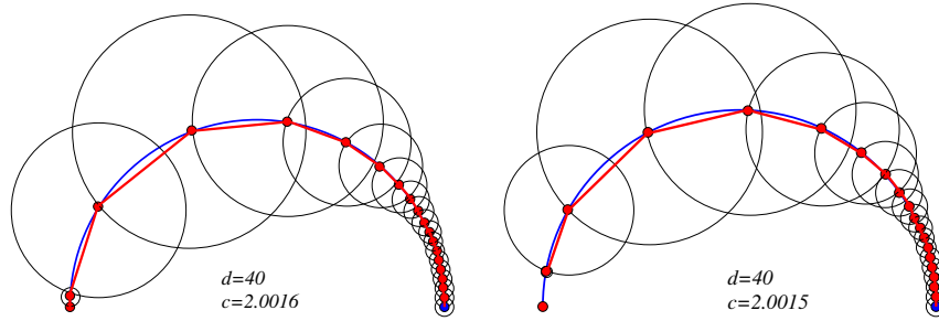
Fig. 5. An example for d = 40 , with starting point on the right, corner on the left of the semi-circles: (Left) For c = 2.0016 , the circle sequence reaches the corner, showing that the chosen c can be achieved. (Right) For c = 2.0015 , the sequence collapses before reaching the corner, showing that the chosen c cannot be achieved. The actual optimum is about 2.001525\dots
