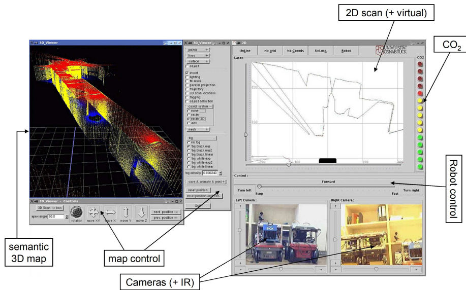
Fig. 1. The user interface for controlling the mobile robot Kurt3D. The left part shows the 3D map, with semantically labeled points (blue for floor points, yellow for wall points, red for ceiling points) and the OpenGL controls. The right part shows a local virtual 2D scan, two camera images and the measurement of the CO 2 sensor. The left camera image corresponds to the left pan and tilt camera, the right image can be switched between camera and IR camera.
