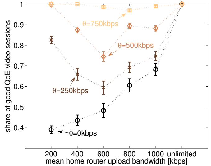
Fig. 5. Share of requests receiving a good QoE.
