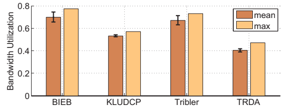
Fig. 6. Bandwidth utilization compared to the theoretical maximum
