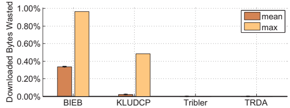
Fig. 7. Amount of wasted data downloaded but discarded during playback
