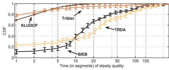
Fig. 3. Inter Switching Times CDF
