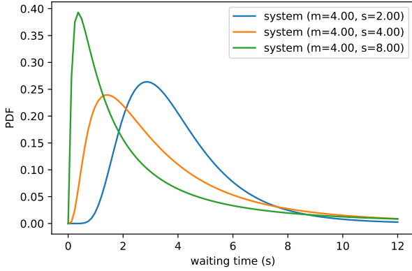
Fig. 2. Web QoE example : The three curves indicate different systems with same mean waiting time of m = 4 s, but varying standard deviation s which impacts the tail of the distribution.
