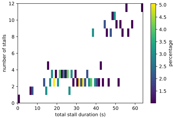
Fig. 4. Video example : Empirical joint probability mass function h(n, t) of the QoS conditions (i.e. number n of stalls and total stall duration t ) for a scenario with a packet loss ratio of 9.6%. The color indicates the joint probability h(n, t) .
