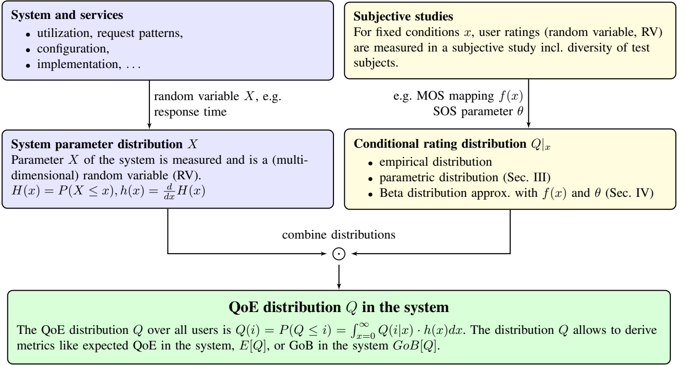
Fig. 1. Overview on system QoE (being observed in a real system) and user rating distributions in a subjective study.
