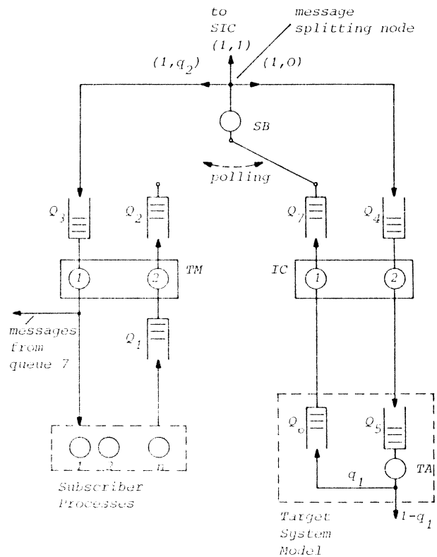
Fig. 4 Queueing Model for the Universal Environment Simulator UNES
