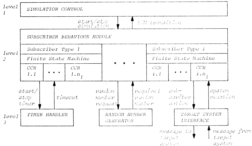
Fig. 3 Software Structure of the Universal Environment Simulator UNES (CCR : Call Control Record)
