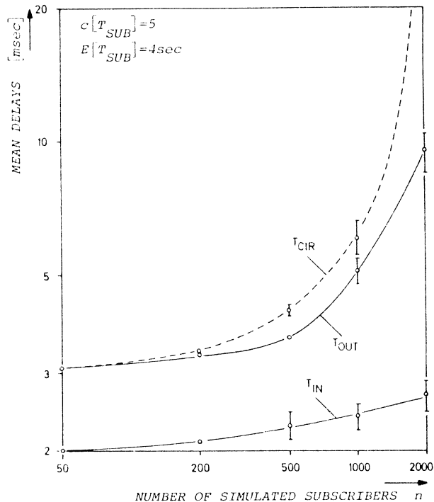
Fig. 6 Mean Delays vs Number of Simulated Subscribers
