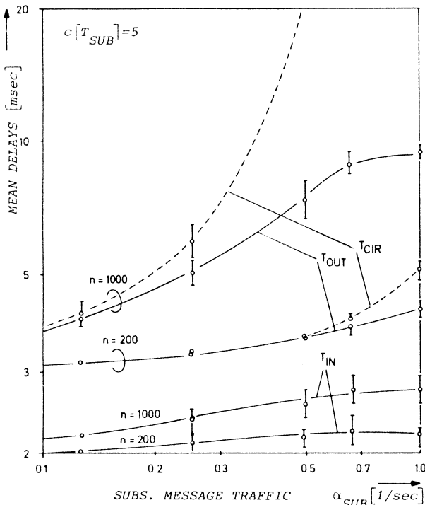
Fig. 5 Mean Delays vs Subscriber Message Traffic Intensity
