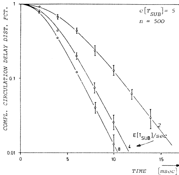
Fig. 7 Complementary Circulation Delay Distribution Function
