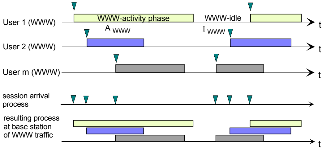
Figure 7 Resulting HTTP traffic process at base station
