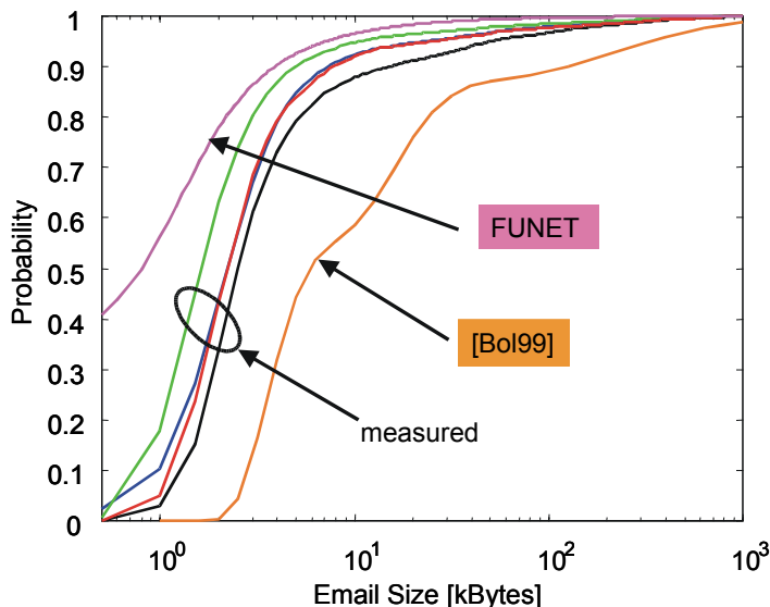
Figure 3 Cumulative distributions of E-Mail sizes
