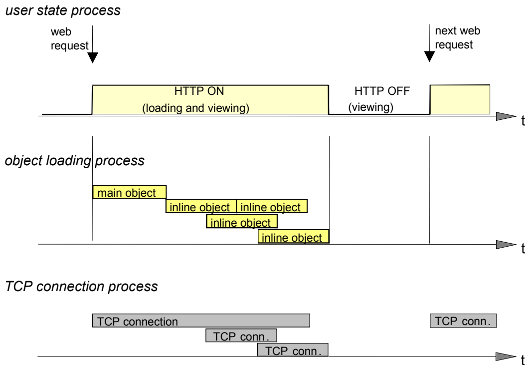
Figure 2 Behavioral user model of Choi
