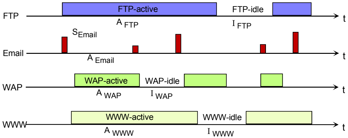
Figure 5 Single user behavior model
