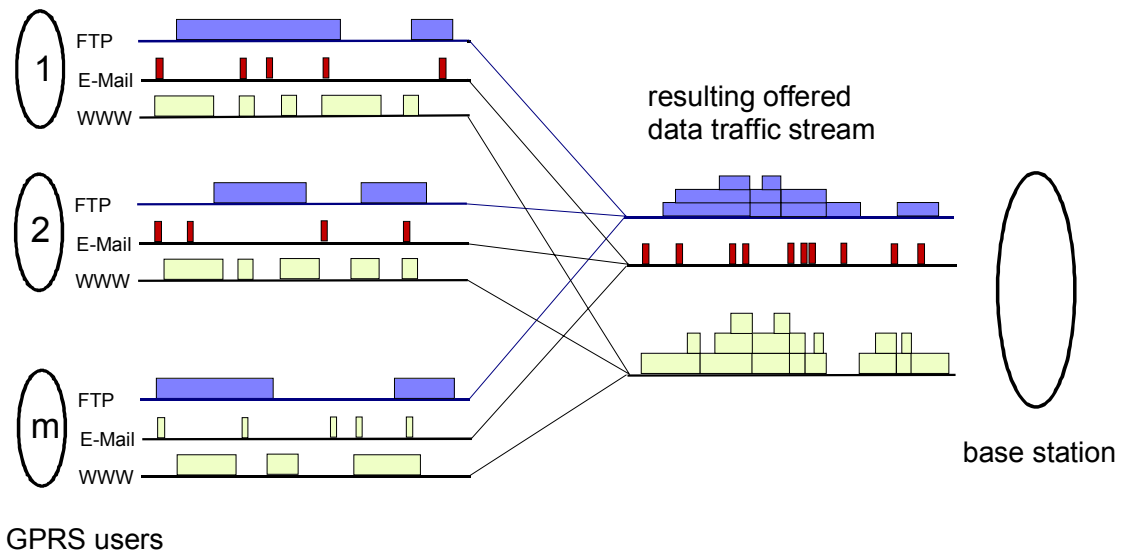
Figure 4 Finite source arrival process
