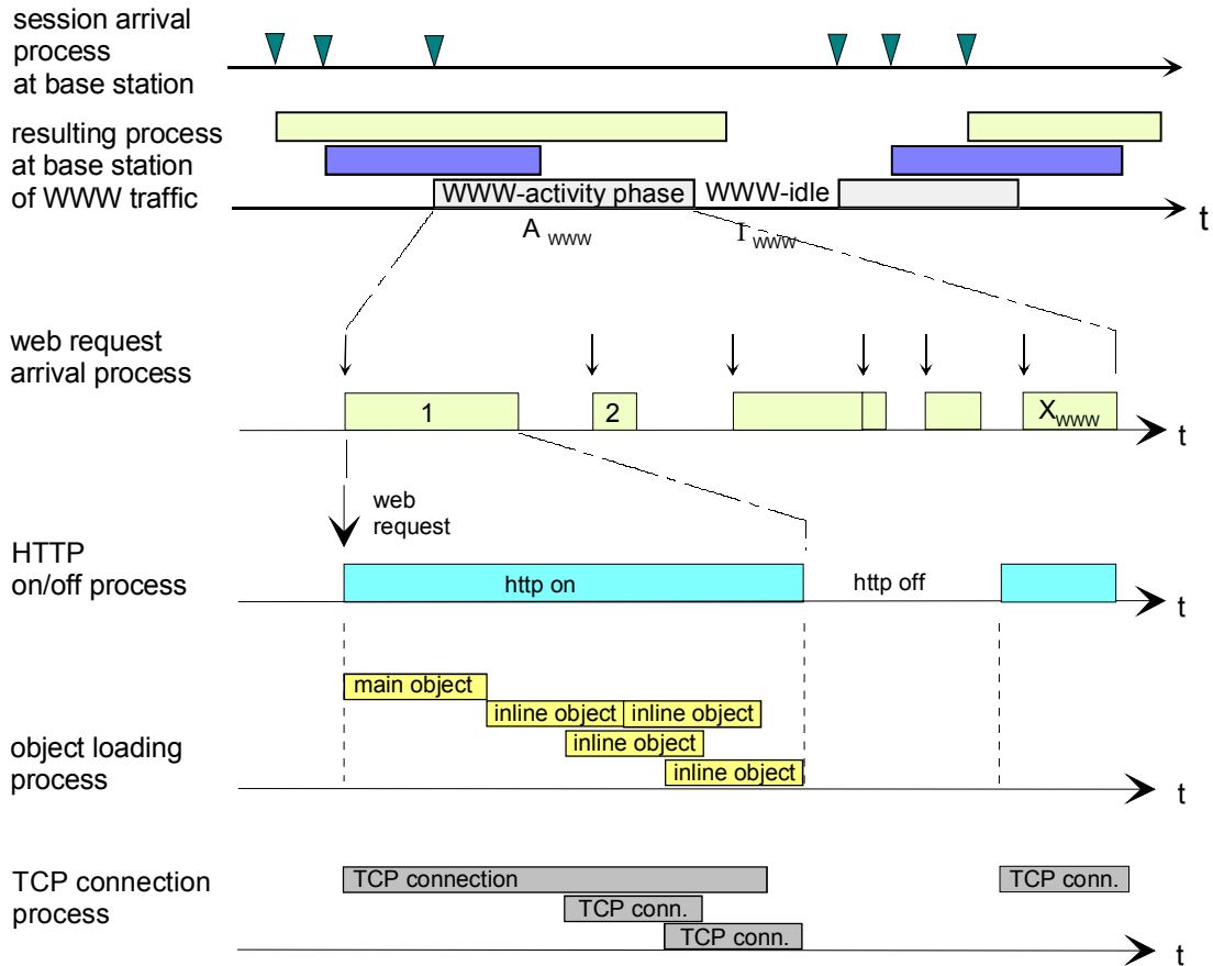
Figure 8 WWW activity phase
