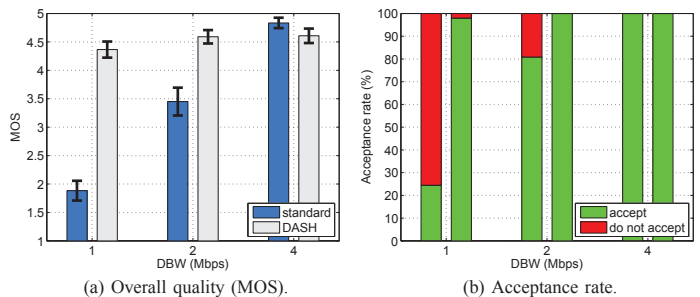
Figure 3. Overall quality and acceptability in YouTube standard (i.e., non-DASH) and DASH. DASH is capable of handling lower DBW connections with high QoE, trading image quality by lower download throughput.
