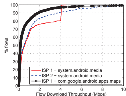
Figure 22. Network neutrality and identification of traffic differentiation. End-device throughput measurements can be used to identify potential traffic differentiation policies done by an ISP, based on types of traffic.
