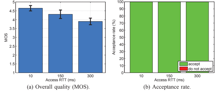
Figure 9. QoE in Facebook. Overall quality and acceptability for different access RTT configurations.
