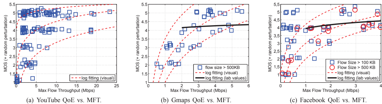
Figure 17. QoE for YouTube, Gmaps and Facebook in the field. Squares and circles correspond to individual sessions reported/rated by participants. Red/black lines correspond to log fitting curves. Filtering out small flows improves the correlations between flow throughput measurements and QoE, specially by avoiding protocol impact on the achieved downlink speed.
