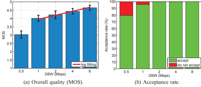
Figure 6. QoE in Facebook. Overall quality and acceptability for different DBW. A DBW of 1 Mbps is high enough to achieve good QoE and almost full acceptability.
