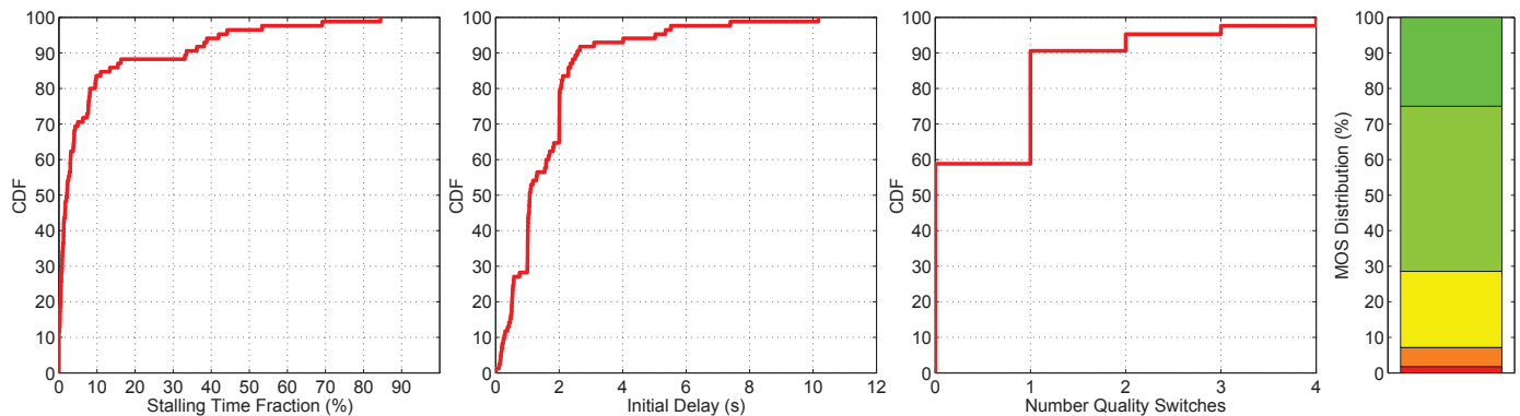
Figure 19. Using YoMoApp to monitor YouTube in smartphones. Results correspond to the monitoring of one single participant. Quality is good (i.e., MOS \geq 4 ) for about 70% of the video sessions, with an initial playback delay below 2 seconds, a total stalling fraction below 4%, and with almost no quality switches for these sessions.
