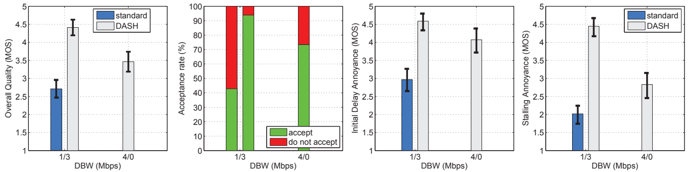
Figure 11. QoE in YouTube under bandwidth fluctuations. Overall quality, acceptability, and annoyance caused by initial delays and stalling for 1/3 (average downlink bandwidth = 1.5 Mbps) and 4/0 (average downlink bandwidth = 2.7 Mbps) downlink bandwidth profiles.
