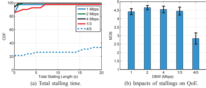
Figure 14. Monitoring of stalling and their impact on QoE with YoMoApp.
