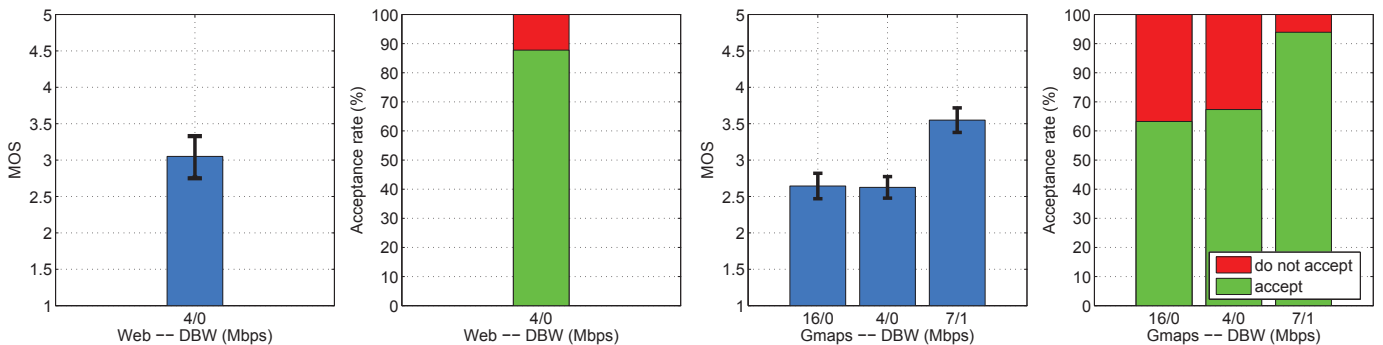
Figure 12. QoE in Gmaps and Web browsing under bandwidth fluctuations. Overall quality and acceptability for different downlink bandwidth fluctuation profiles. Bandwidth outages have a very marked impact on the QoE of these services, and higher downlink bandwidth values do not compensate for such drops.
