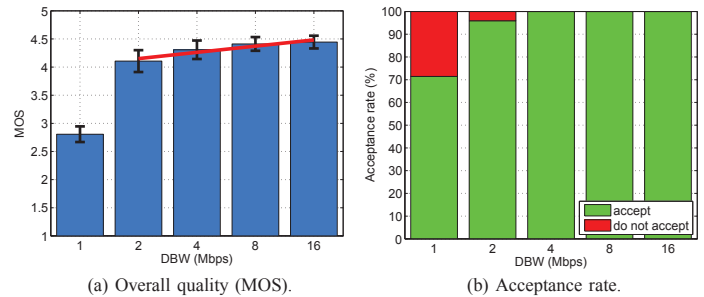
Figure 5. QoE in Gmaps. Overall quality and acceptability for different DBW. A DBW of 2 Mbps is high enough to achieve good QoE and almost full acceptability.
