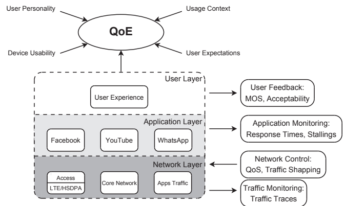
Figure 1. Layered QoE evaluation methodology for networking services.
