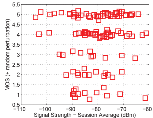
Figure 18. MOS vs signal strength in YouTube. The signal strength metric corresponds to the average single strength when considering all the flows of a single session. There is no apparent correlation between the MOS declared by participants and the measured average signal strength.
