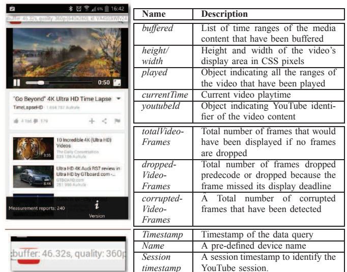
Figure 13. Screenshot of the app and selected parameters from the HTML5 <video> object, Media Source Extensions, and device, which can be tracked by the app.
