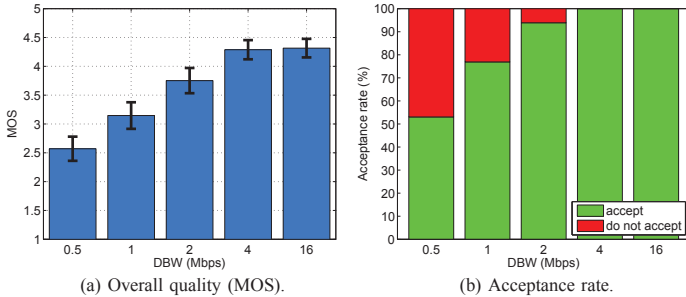
Figure 8. QoE in WhatsApp. Overall quality and acceptability for different downlink bandwidth configurations.
