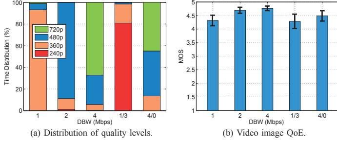
Figure 15. Monitoring of video quality switches and the resulting image QoE with YoMoApp.
