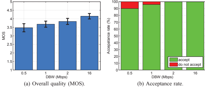
Figure 7. QoE in Web browsing (news website). Overall quality and acceptability for different downlink bandwidth configurations.
