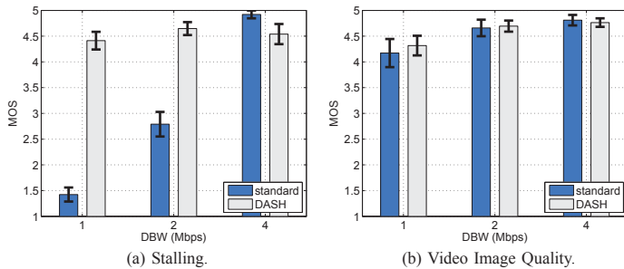
Figure 4. QoE for YouTube Mobile, considering playback stalling and video image quality. Video image quality is perceived as almost excellent for the lowest DBW condition, even if video resolution is lower.
