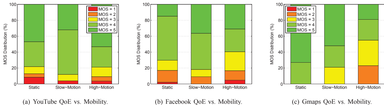
Figure 20. Potential impact of mobility on overall QoE. Mobility patterns are constructed based on location as declared by participants when performing the evaluation tasks. Static refers to locations “home” and “office”, slow-motion refers to location “street”, whereas high-motion refers to locations “car”, “metro” and “train”.
