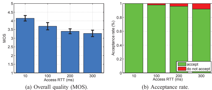
Figure 10. QoE in Web browsing (news website). Overall quality and acceptability for different access RTT configurations.
