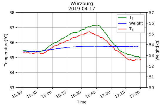
(a) Swarm-like anomaly in sensors T 6 and T 8 , but not within the measured weight.
