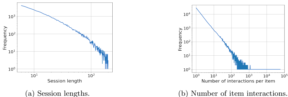
Fig. 2: Different frequency distributions for the Fashion dataset.
