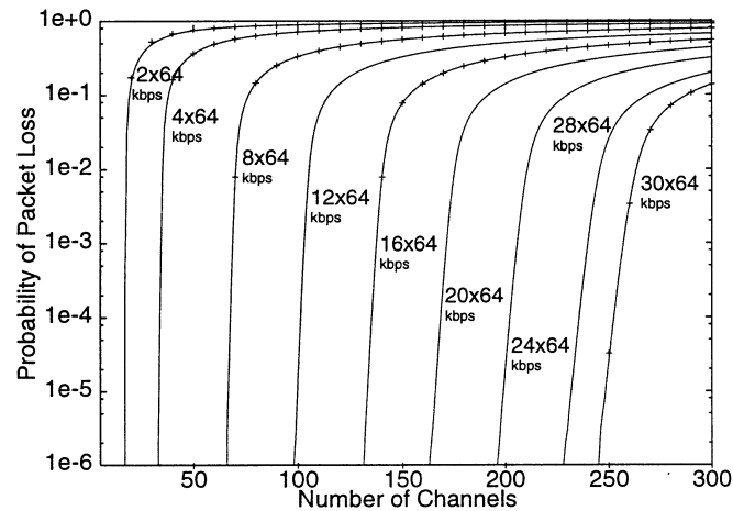
Figure 4: Packet Loss Probability
