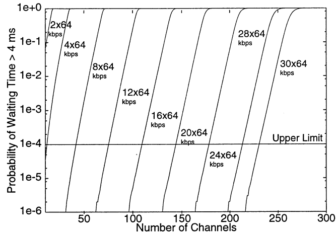
Figure 3: Complementary Packet Delay Distribution
