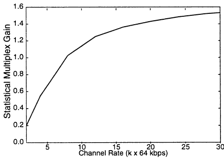
Figure 5: Statistical Multiplexing Gain
