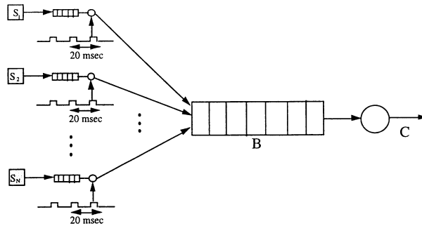
Figure 1: Voice Path from Mobiles to the BS-MSC link
