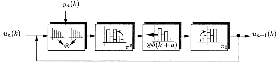
Figure 2: computational diagram for buffer occupancy distribution
