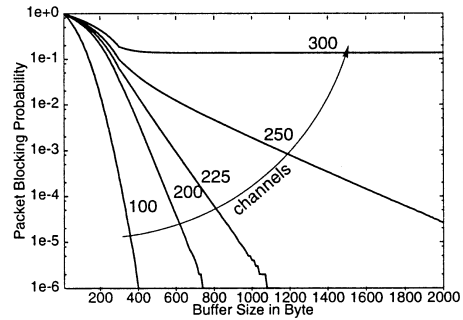
Figure 6: Buffer Size
