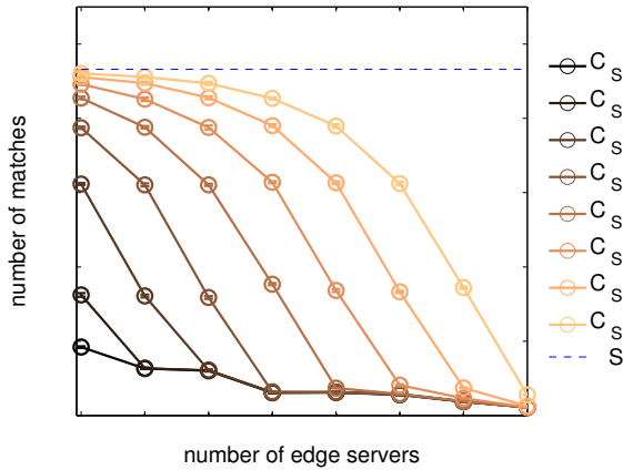
Figure 10: Effect of C_{ES} on the DS load.
