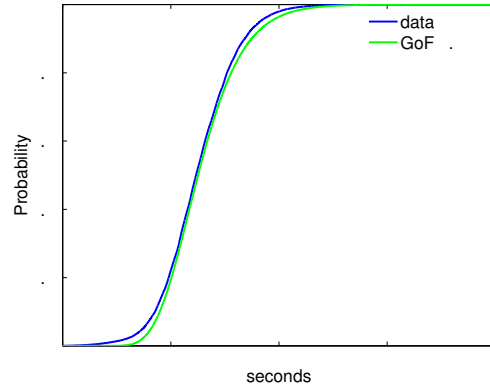
Figure 5: CDF of match durations in Valve’s EU West server.
