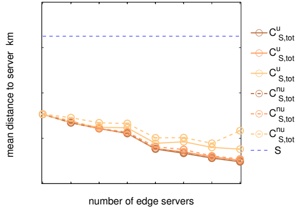
Figure 11: Effect of fixing the C_{ES,tot} on the mean distance to server.
