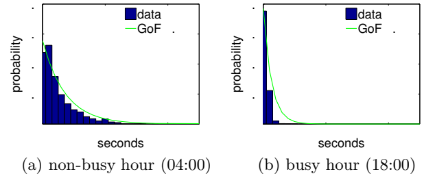
Figure 3: EU West server inter-arrival times
