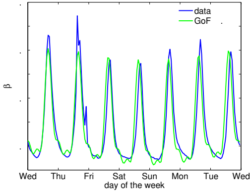
Figure 4: \beta dynamics in EU West server.
