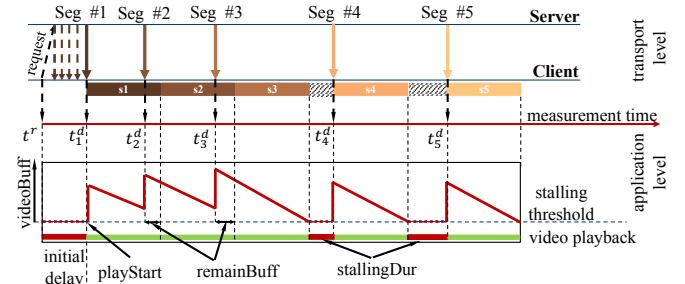
Fig. 1. Graphical View of Estimating Video Quality Algorithm
