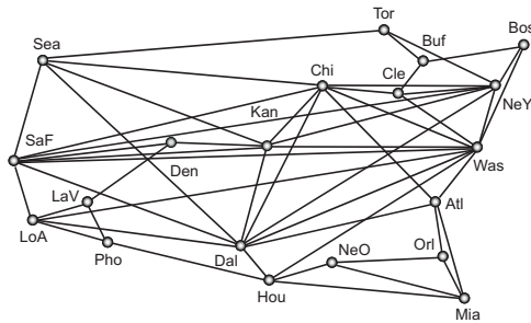
Figure 5: Topology of the Labnet03 network with 20 nodes and 53 bidirectional links.
