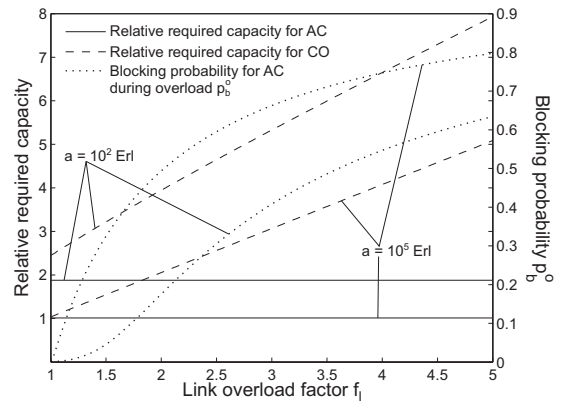
Figure 4: Impact of the overload factor f_l on the required capacity and the blocked traffic of a single link for a = 10^2 and 10^5 Erlang.
