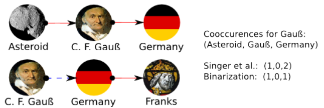
Fig. 2: Illustrative example of the semantic extraction methods. With [6] and a window size of 2, the pair ( Gauß , Germany ) would have been counted twice (all arrows), whereas we ignore the second occurrence of this pair (blue dashed arrow) and only count the unique pairs (red solid arrows).
