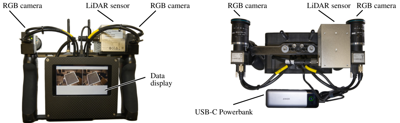
Figure 2. Backside and top of the proposed handheld mapping system for data collection.
