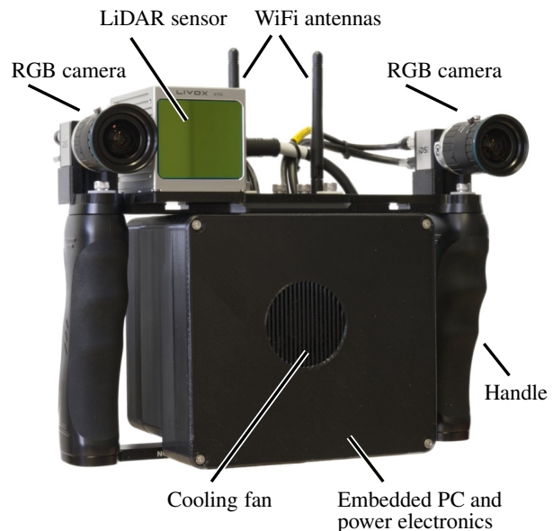
Figure 1. Proposed handheld mapping system with stereo RGB cameras and Livox Avia LiDAR sensor.
