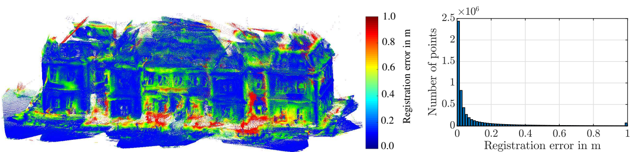
Figure 7. Point cloud of the result from 15 scans using depth map completion compared to the reference scan created using scan matching from 3000 scans. Left: Completed point cloud colored by distance to the reference cloud with corresponding colorbar. Right: Corresponding error histogram of the cloud-to-cloud distance.
