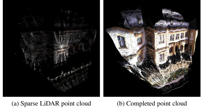
Figure 5. Comparison of sparse input and completed point cloud. Left: Sparse LiDAR point cloud with 17.627 points. Right: Completed point cloud with 401.687 points.
