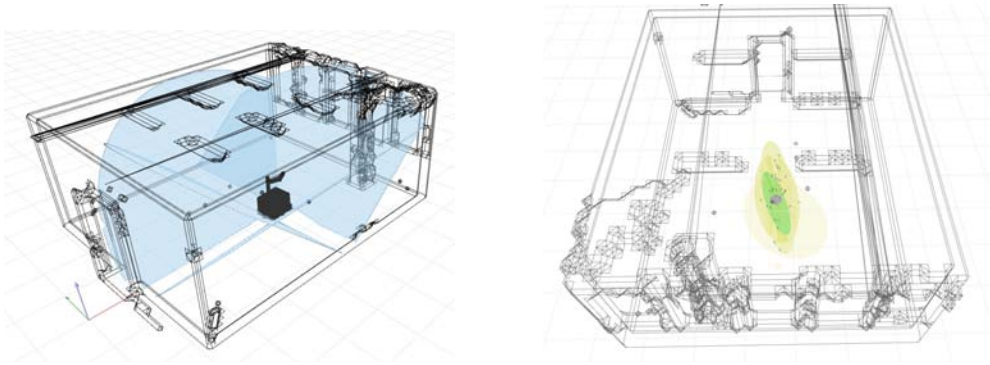
Figure 9: Application example: Ray tracing for localization in polygonal maps. For this purpose, only the extracted polygons were used, not the retesselated map. The used robot is equipped with several laser scanners mounted at fixed angles and pointing at different directions. A Ray tracing technique is used to calculate a sensor model (left). The right figure shows the improvement of the self localization. The yellow area marks the estimated pose error without the use of the tilted scanners. The green area shows the result using the additional information from these scanners. The localization improves considerably [13].
