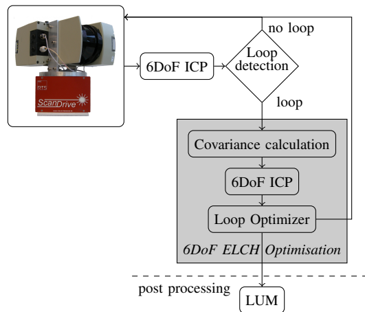
Fig. 2. Schematic overview of the complete algorithm, namely the interaction of ICP, ELCH and LUM. The dashed line separates the global optimization part that is executed as a post processing step.
