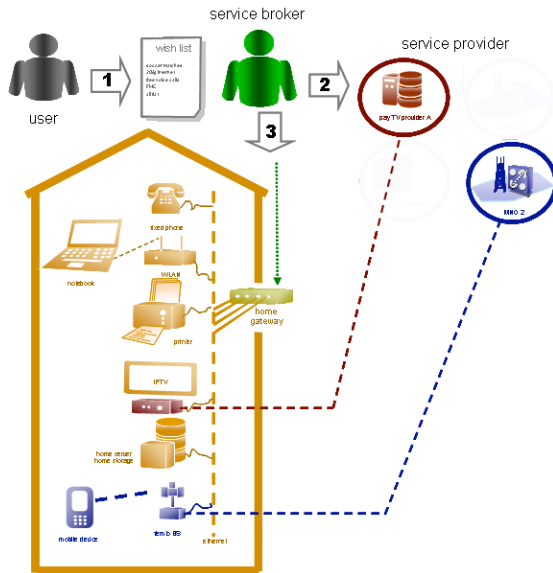
Fig. 2. Service Broker
