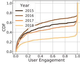
Figure 6: Evolution of user engagement.
